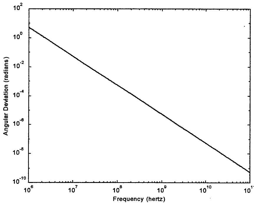
Figure 67. Angular deviation due to spatial TEC variation
