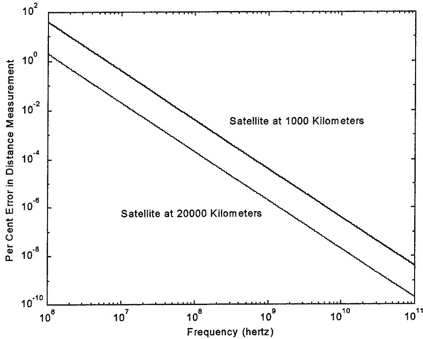
Figure 64. Distance measurement errors from two satellites
