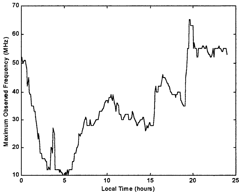
Figure 81. Maximum observed frequencies over 24 hours at Oahu.
