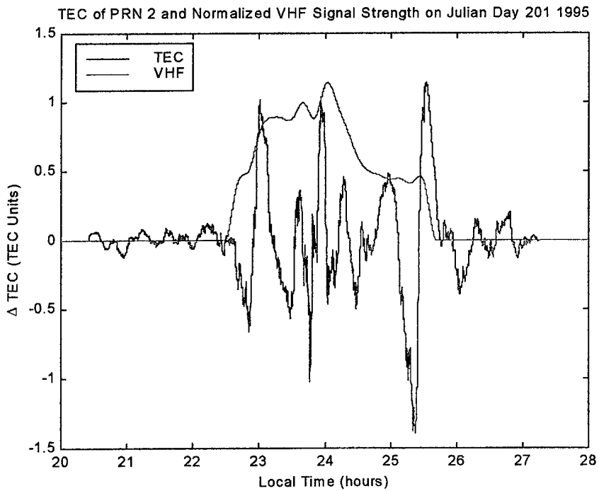
Figure 49. \Delta TEC and normalized VHF signal strength on day 201.
