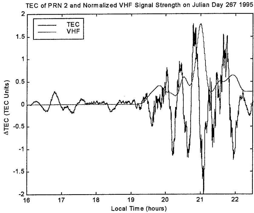
Figure 48. \Delta TEC and normalized VHF signal strength on day 267.
